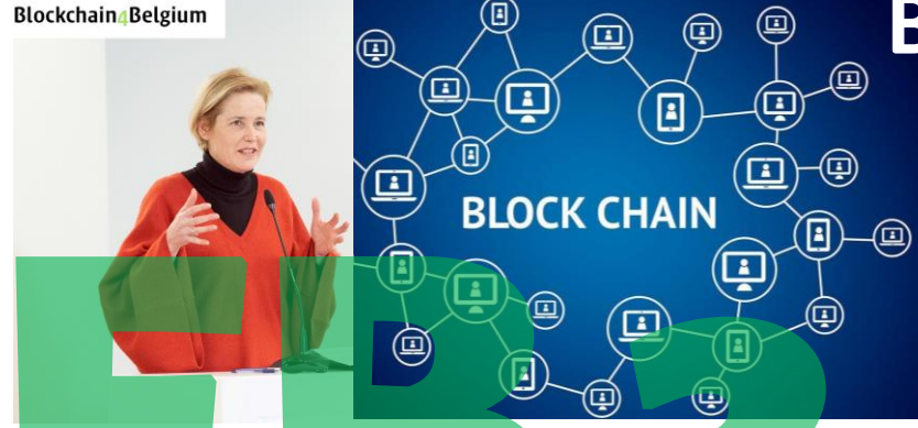
Blockchain
